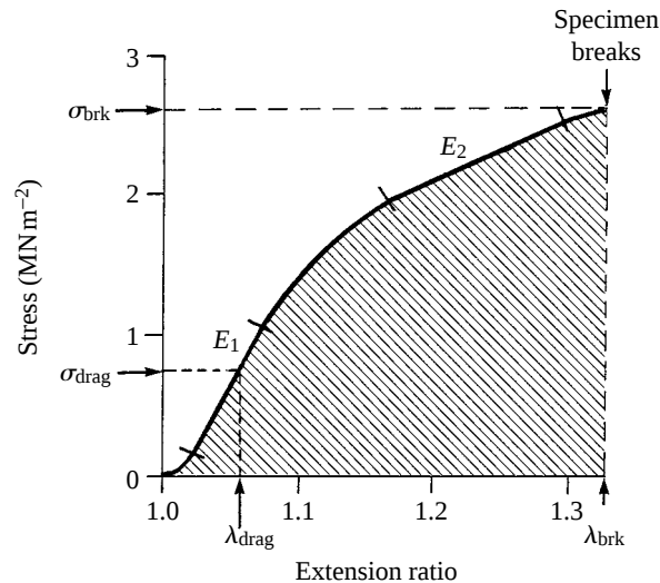
Fig. 2. Plot of stress ( \sigma ) as a function of extension ratio ( \lambda ) for a piece of the stipe of N. luetkeana from the protected site subjected to a tensile test. \sigma_{brk} , stress required to break the stipe; \lambda_{brk} , extension ratio required to break the stipe; \sigma_{drag} , stress in the stipe due to drag on the kelp in a current of specific velocity; \lambda_{drag} , extension ratio due to this drag; E_1 , elastic modulus of the stipe tissue at low \lambda ; E_2 , elastic modulus at high \lambda . The hatched area under the curve indicates the work per tissue volume ( W/V ) required to break the specimen.
