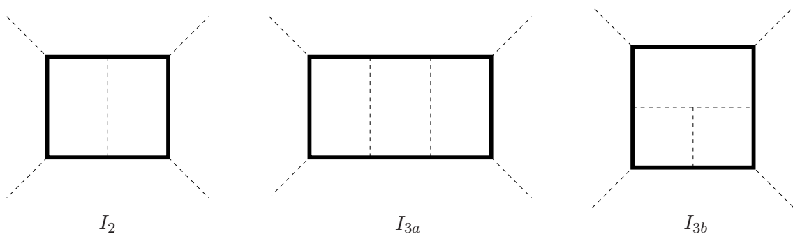
Figure 3. Two- and three-loop four-point dual conformal diagrams. I_2 and I_{3a} are ladder diagrams; I_{3b} is the tennis-court diagram. Numerator factors (including a loop-momentum-dependent factor for the tennis court) are omitted. See eqs. (A.20) and (A.23) for explicit formulae for the integrals.
