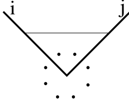
Figure 1. The one-loop eikonal diagram contributing to S_n^{(1)} . A graviton (thin line) is exchanged between external legs i and j (thick lines). The dots signify an arbitrary number of other external legs.
