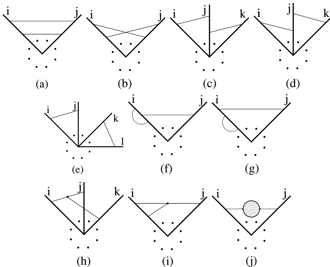
Figure 2. Two-loop eikonal diagrams contributing to S_n^{(2)} .
