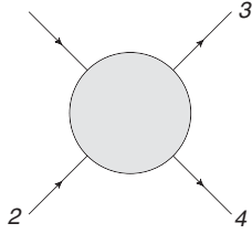
FIG. 1. Particle labels used throughout for 2 \rightarrow 2 scattering.
