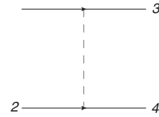
FIG. 2. The Regge limit as two Wilson lines separated by a transverse distance z .
