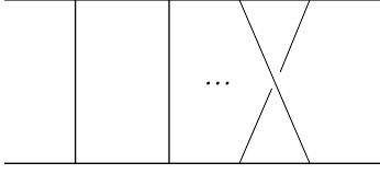
Fig. 2. A representative (crossed) ladder graph, where all particles are gravitons. The sum of all such diagrams in the leading Regge limit builds up the exponentiated amplitude of eq. (2.8).
