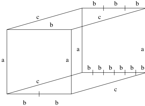
Figure 3 The analogous building block for \Gamma(2, 3)
