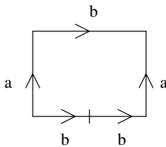
Figure 2 The “horobrick” building block for the geometric model of BS(1, 2)
