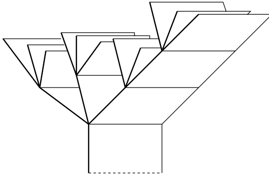
Figure 1 The geometric model of the solvable Baumslag–Solitar group BS(1, 3) , which is topologically a warped product of a tree and \mathbb{R}
