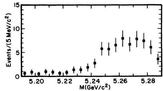
FIG. 10. The mass distribution for partially reconstructed B^0 \rightarrow D^{*+}\pi^- candidates, obtained from a Monte Carlo simulation of B^- \rightarrow D^{*0}(2420)\pi^- , D^{*0}(2420) \rightarrow D^{*+}\pi^- events. The number of events is normalized to a product branching fraction of 0.14%.
