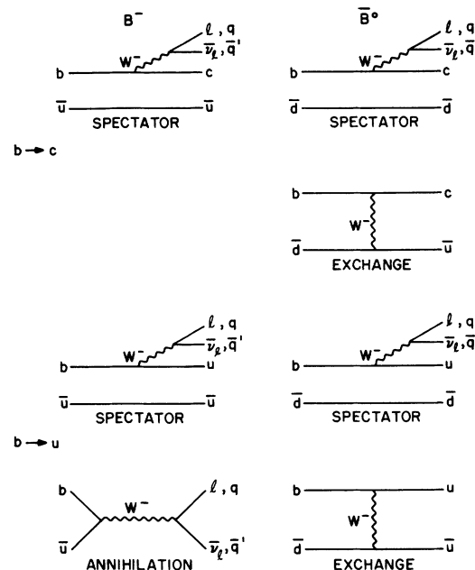
FIG. 1. The spectator, exchange, and annihilation diagrams for B^- and \bar{B}^0 decay. Note that semileptonic decay widths are completely dominated by the spectator diagrams because the exchange diagrams do not produce leptons and the annihilation diagram for B^- decay is strongly Cabibbo-suppressed since it involves a b \rightarrow u transition. If the exchange contributions are important, the B^- and \bar{B}^0 lifetimes would be different, resulting in different semileptonic branching fractions for B^- and \bar{B}^0 decays.
