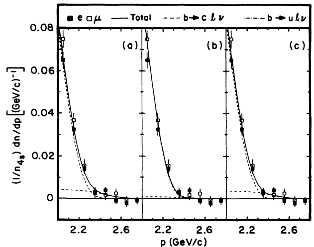
FIG. 7. The electron and muon momentum spectra in the interval, 2.0 \leq p_\ell \leq 2.8 GeV/c; (a) is the fit to the ACCMM model, (b) is the fit to the ISGW model, and (c) is the fit to the ISGW** model where the D^{**} fraction is allowed to vary. The b \rightarrow c\ell\nu and b \rightarrow u\ell\nu components are shown along with the total. The b \rightarrow c \rightarrow s\ell\nu contribution is negligible in this momentum interval and has not been included in the figures.
