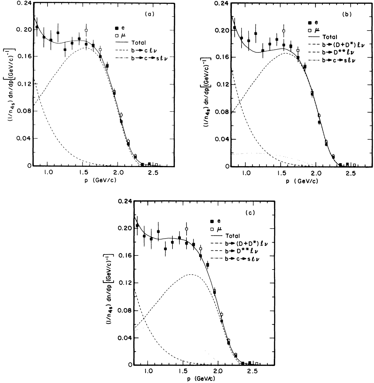
FIG. 6. The electron and muon momenta spectra for p_\ell \geq 0.8 GeV/c and the fits to these data; (a) is the ACCMM fit, (b) is the ISGW fit, and (c) is the ISGW** fit where the D^{**} fraction is allowed to vary. The total fit and the b \rightarrow c\ell\nu and b \rightarrow c \rightarrow s\ell\nu components are illustrated as indicated. For clarity, the b \rightarrow u\ell\nu components are not included.
