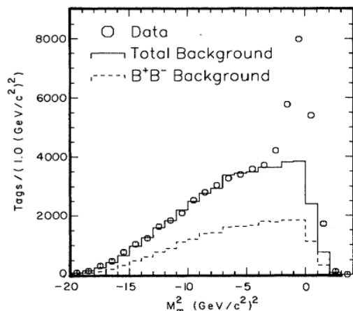
FIG. 1. M_m^2 distribution in data (open circles; error bars are typically smaller than circles), with random components overlaid as estimated by Monte Carlo simulation from B^-B^+ events (dashed histogram) and total (solid histogram).
