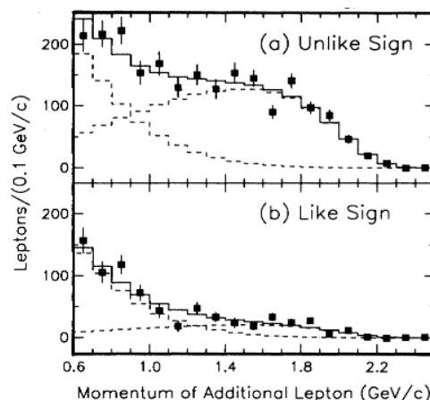
FIG. 2. Efficiency-corrected spectrum of additional leptons in tag events, for (a) opposite-sign and (b) same-sign leptons. Superimposed are fits (solid) to a primary lepton spectrum (dashed) plus a secondary spectrum (dash-dot) (see text).
