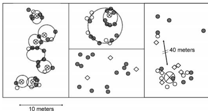
Fig. 3. A selection of four genets that demonstrate the range of Sequoia sempervirens clonal structures found in the Jackson Demonstration State Forest, north coast of California, including (a) chains of overlapping rings on site S2, (b) concentric rings on site S1, (c) disjunct stems on site R1, and (d) distantly disjunct stems on site N2. Solid circles represent ramets from a single clone. Open circles represent trees not sampled, open diamonds represent single stem genets, crossed circles represent stumps, and dotted circles outline perceived fairy-rings.
