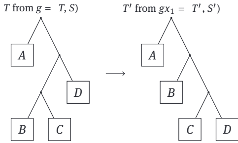
Figure 6. If g = (T, S) and gx_1 = (T', S') , where the tree T contains at least a root caret whose right child has a left child, the combinatorial rearrangement of the subtrees of T yielding T' . Here, A, B, C and D represent possibly empty subtrees and S = S' .
