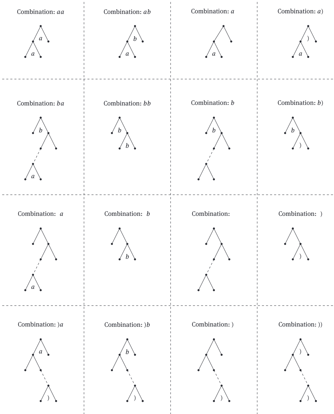
Figure 4. Every possible pair of caret labels in L_{\text{int}} and the relative placement of the carets they encode.
