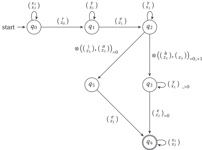
Figure 7. For \otimes u, v as in Case 5, this machine checks that the change in the root caret of subtree C from T to T' occurs in the correct spot in the string and has the correct label change. The edge labels correspond to the letters in the string v = v g x_1 \in \mathcal{F} and the corresponding letter from u = v g is ignored, except at the root caret of subtree C , where both the letter from u and from v are considered. The letters z_0, z_1, z_2 are as in the expressions for u and v above, y \in \Sigma_{\text{int}} and x_i \in \Sigma_T . The start state is q_0 and the accept state is q_4 . The letter \mathcal{J} denotes the set of counter instructions used in the construction of \text{int} .
