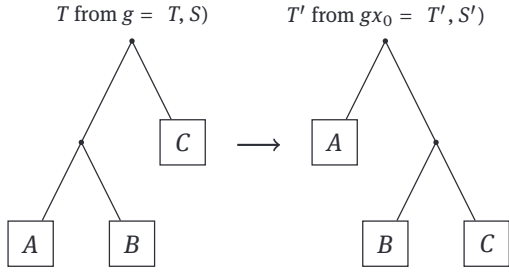
Figure 5. Part of the tree pair diagrams for g = (T, S) and gx_0 = (T', S') . The letters A, B, and C represent possibly empty subtrees, and S = S' .
