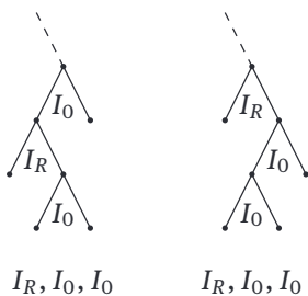
Figure 1. Fordham’s caret labels are not in bijective correspondence with binary trees: two different interior subtrees corresponding to the same string of labels. Labels are listed in infix order.
