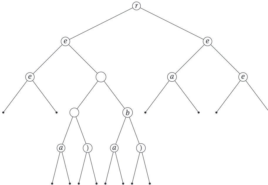
Figure 2. An example of a tree corresponding to the string of labels eea ) ab)raee .
