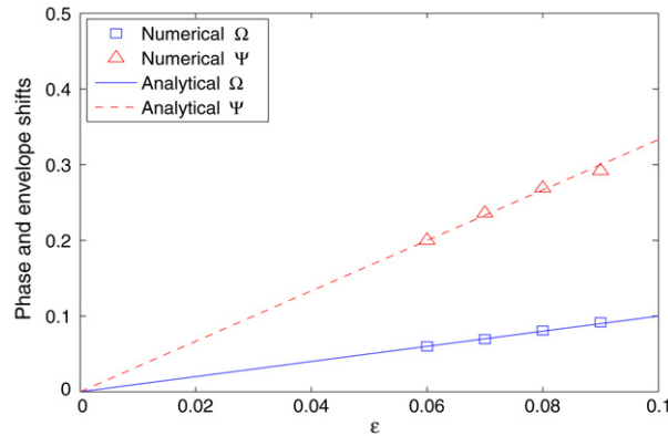
Fig. 3. Plot of numerically computed phase and envelope shifts (markers) and the analytical values (lines); both shifts are O(\varepsilon) and the analytical shifts are close to the computed ones.
