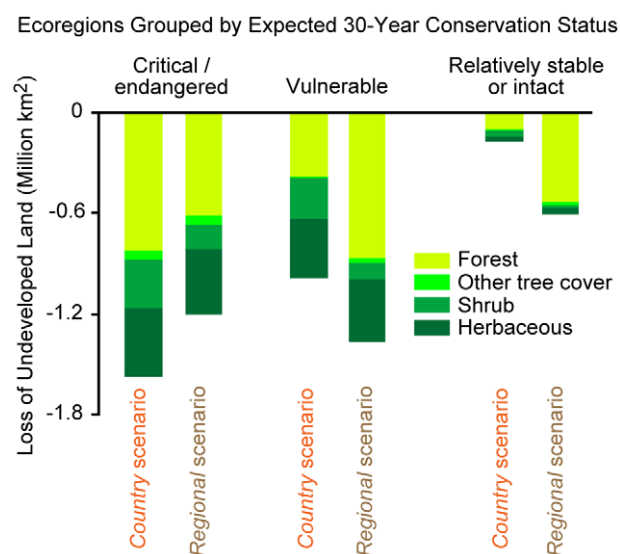
Figure 7. Projected global change in undeveloped land area from 2000 to 2015 by ecoregion status. Each bar indicates the loss of undeveloped land area by vegetation type [109]. See the text and [84] for more information on ecoregion status. In this graph we do not include any undeveloped land area provided by cropland abandonment from 2000 to 2015.
