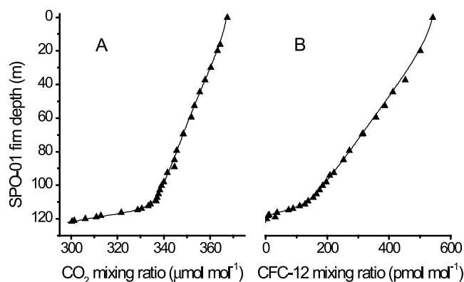
Figure 1 (a) Firn air measurements of \text{CO}_2 (solid triangles) from SPO-01 compared with model simulations (solid line). (b) Firn air measurements of CFC-12 from SPO-01 (solid triangles) compared with model simulations (solid line).
