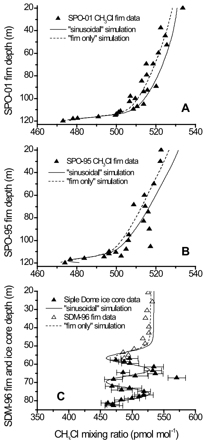
Figure 3 Depth profiles of \text{CH}_3\text{Cl} ice core data and firn air measurements, compared with model simulations based on the “firm only” and “sinusoidal” atmospheric histories shown in Figure 2: (a) South Pole (SPO-01), (b) South Pole (SPO-95), and (c) Siple Dome (ice cores, and SDM-96); the error bars represent the uncertainty in the ice core data. Results from the top 20 m of the firn are omitted because they are subject to seasonal variability. Note that the general trends in all firn data are correctly simulated with the “sinusoidal” history.
