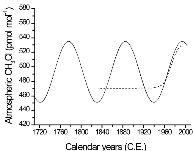
Figure 2 Atmospheric histories for \text{CH}_3\text{Cl} derived from firn air and ice core data: “firn air only” history developed to fit the SPO-01 \text{CH}_3\text{Cl} data (dashed line) and “sinusoidal” history (solid line). The “firn air only” history extends back 170 years but it is very loosely constrained by the firn data for the period before 1900 C.E. The “sinusoidal” history does not represent a fit but rather a close approximation to the amplitude and period observed in the ice core data.
