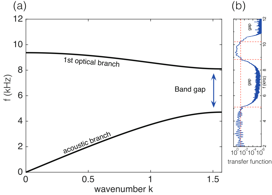
Figure 3. Pass bands (acoustic and optical) and band gap for the diatomic granular chain considered in [20]. (a) Analytical expression derived from the corresponding dispersion relations. (b) Experimental transfer function inferred when sending ‘white noise’ from one side through the system and then retrieving (on the other side) only the frequencies that belong to the pass bands (observe that the experimental and theoretical cutoff frequencies are somewhat different.) Reprinted figure with permission from [20], Copyright (2010) by the American Physical Society.
