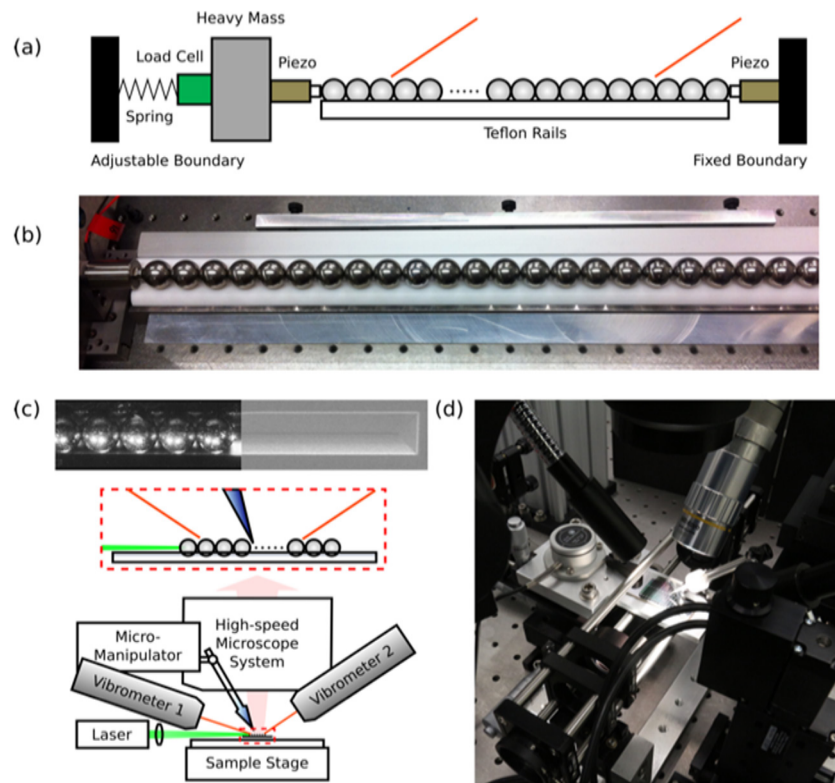
Figure 1. Macroscale and microscale experimental setups for granular chains. (a) Schematic diagram of a typical macroscale setup that includes support rods, boundaries, excitation capabilities, and a detection system. (The orange lines represent laser interferometers, which monitor the displacement and velocity of selected particles.) (b) Laboratory realization of the setup in panel (a) with particles whose diameter is about 1.9 cm. (c) Image and schematic diagram of a typical microscale setup that includes support grooves, robotic manipulation, and optical excitation and detection capabilities. The inset shows an optical image of a granular chain composed of stainless steel particles (of roughly 300 microns in diameter) and a scanning-electron-microscopy image of the support grooves. (d) Laboratory realization of the setup in (c). Panels (a) and (b) used with permission from Paul Anzel. Panels (c) and (d) reprinted figure with permission from [126], Copyright (2016) by the American Physical Society.
