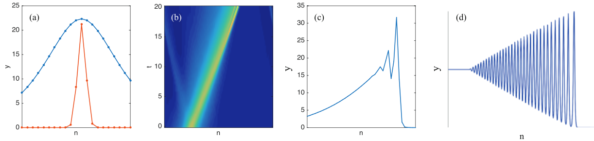
Figure 7. (a) Strain profile of a solitary-wave solution (red curve) in a granular chain. One uses an arbitrary long-wavelength bell-shaped curve (blue curve) as initial data when solving equation (6). (b) Contour plot of the evolution of the blue curve of panel (a) via equation (6). Observe that the high-amplitude portion of the wave (yellow) travels faster than the low-amplitude part (light blue). (c) Strain profile (at time t = 20 ) showing the onset of microscopic oscillations, which are reminiscent of a dispersive shock. (d) Dispersive-shock solution of the KdV equation. Reproduced with permission from [2].
