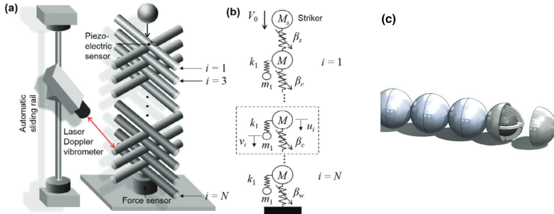
Figure 6. (a) A woodpile chain, which can be modeled as (b) a locally resonant granular crystal. (a) and (b) Reprinted figure with permission from [110], Copyright (2015) by the American Physical Society. (c) A mass-in-mass granular chain. Reproduced with permission from [43].
