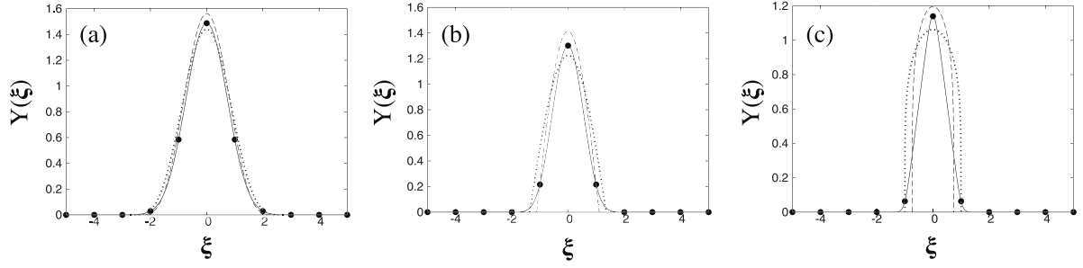
Figure 5. Comparison of continuum approximations and genuine solitary-wave solutions of equation (6) for (a) p = 3/2 , (b) p = 3 , and (c) p = 11 . The markers show the wave on the lattice, dotted curves show the corresponding solutions of the continuum model (23), and dashed curves show equation (16). The approximation does poorer as the nonlinearity exponent p increases. Reprinted figure with permission from [7], Copyright (2009) by the American Physical Society.
