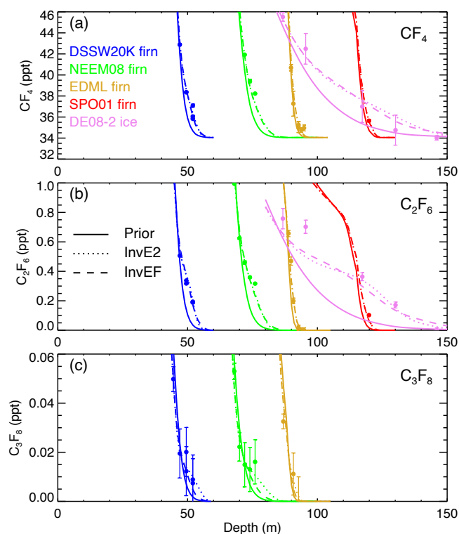
Figure 6. Mole fraction depth profiles at the bottom of the firm and in the DE08-2 ice for (a) \text{CF}_4 , (b) \text{C}_2\text{F}_6 and (c) \text{C}_3\text{F}_8 . Solid lines show mole fraction depth profiles for the prior, dotted lines are InvE2 emissions and dashed lines are for InvEF emission factor. Symbols show measurements with 1\sigma uncertainties.
